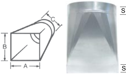
Trans 1 - Square to Round
